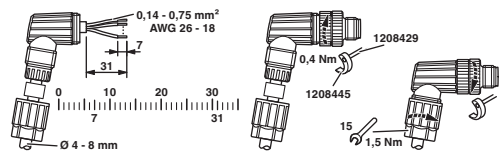
Functional drawing
